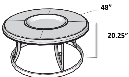
CFP48-K
