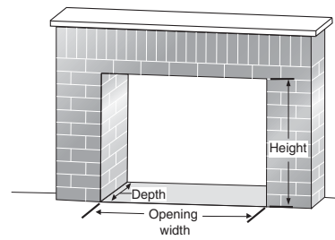
Fireplace Dimensions
