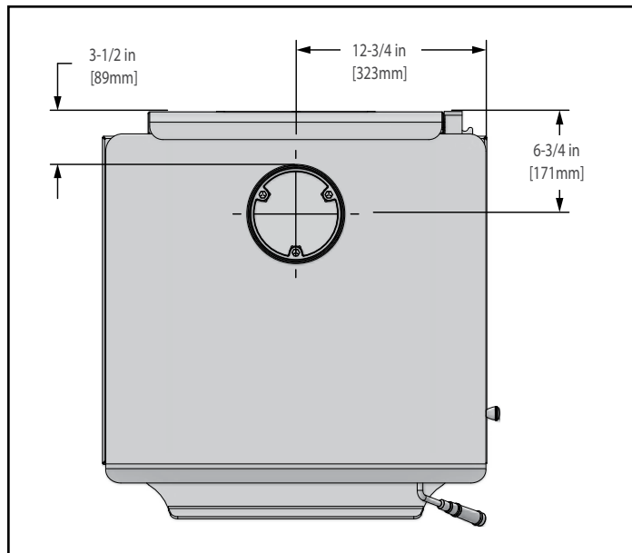
Figure 8.2 - Top View
