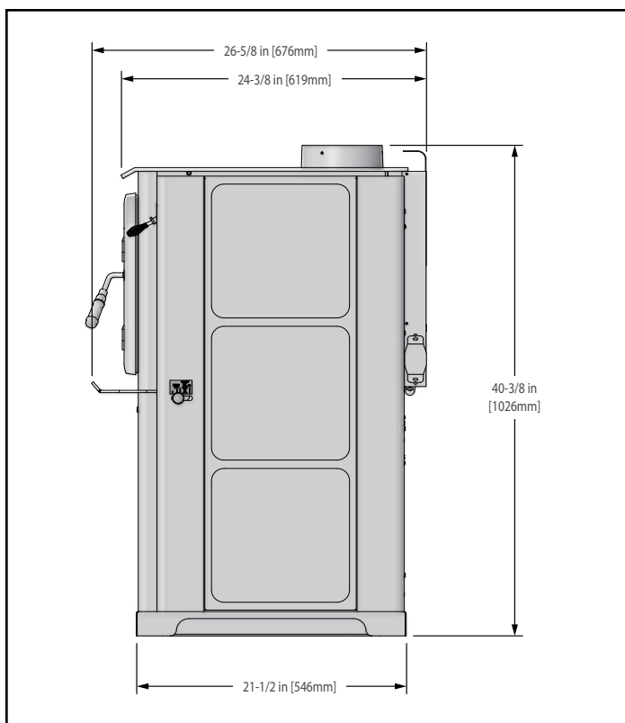
Figure 8.3 - Side View
