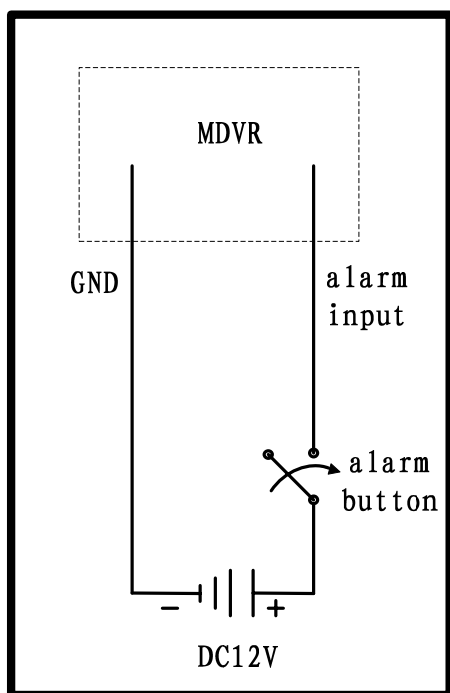
alarm input wiring diagram
