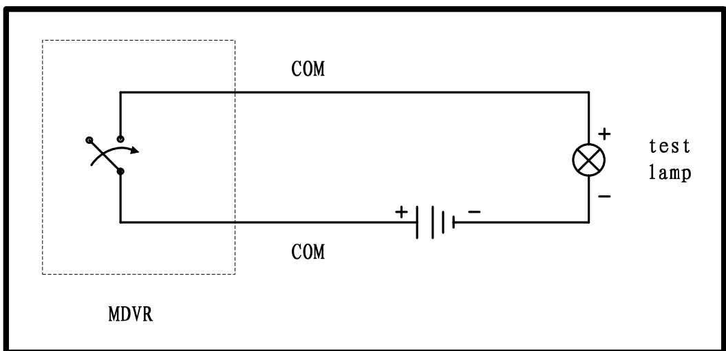
alarm output wiring diagram
