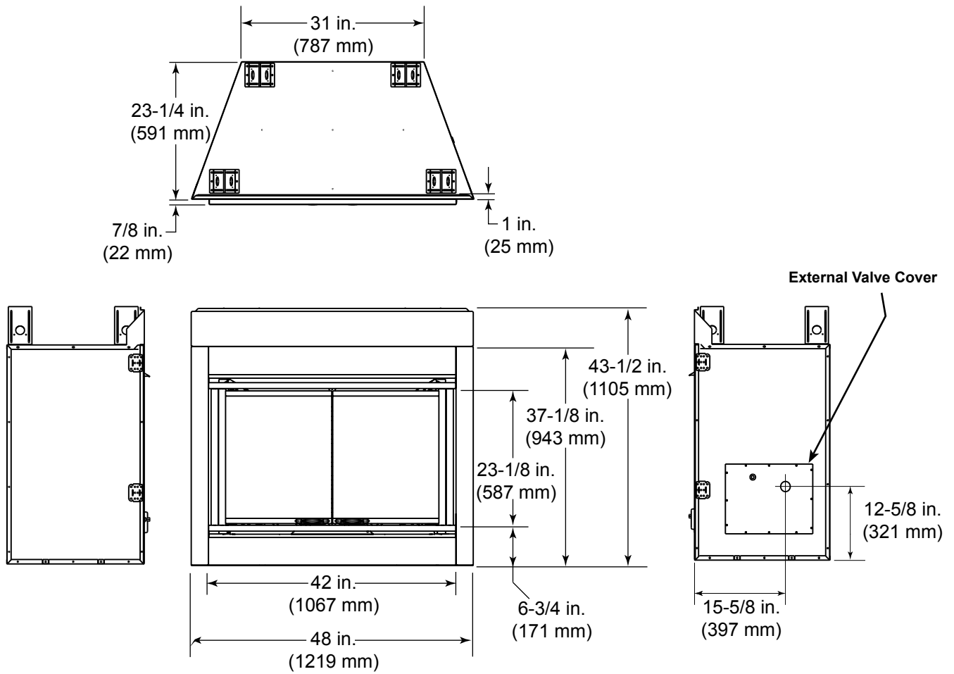
Figure 13.1 Appliance Dimensions
